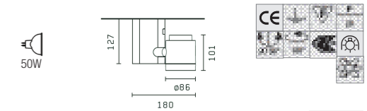
1x MAX 50W QR-CBC 12V Low voltage
