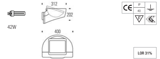
2x 42W TC-TE Compact Fluorescent
