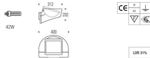
2x 42W TC-TE Compact Fluorescent
