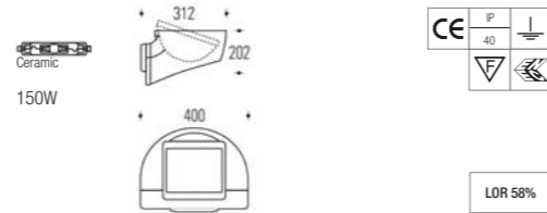
1x 150W DM-TD RX7s Metal Halide
